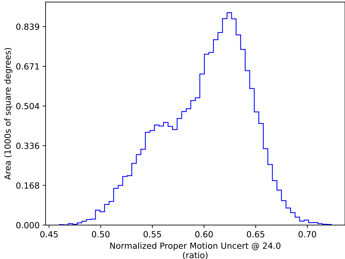
too_elab_r64_d3_gz_v3.4_10yrs WFD: Normalized Proper Motion Uncert @ 24.0
