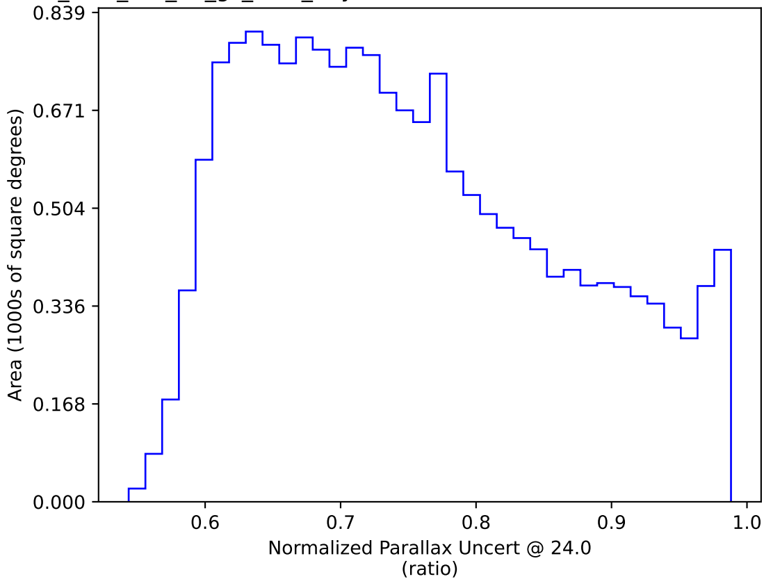
too_elab_r64_d3_gz_v3.4_10yrs WFD: Normalized Parallax Uncert @ 24.0
