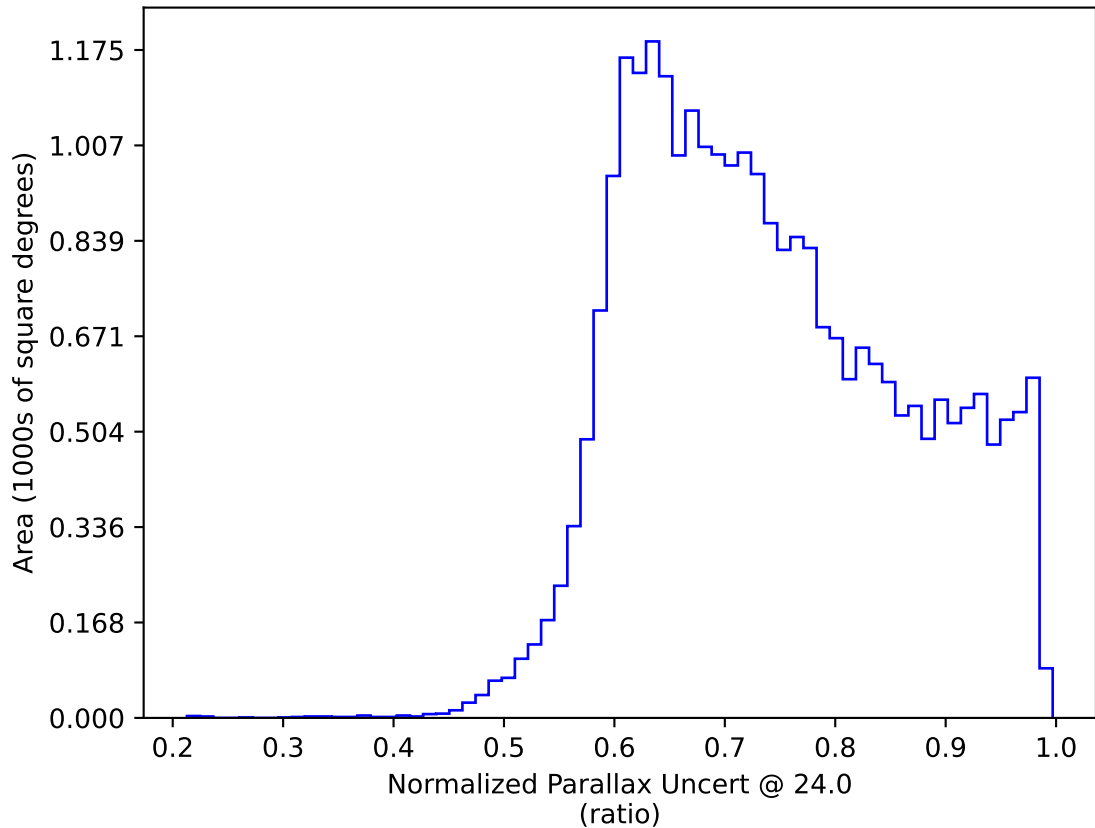
too_elab_r64_d3_gz_v3.4_10yrs All sky: Normalized Parallax Uncert @ 24.0
