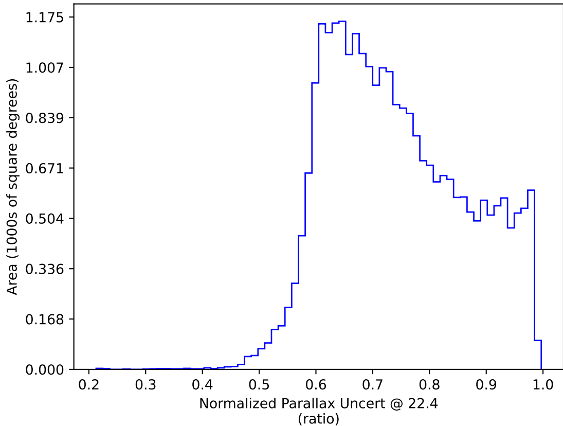
too_elab_r64_d3_gz_v3.4_10yrs All sky: Normalized Parallax Uncert @ 22.4
