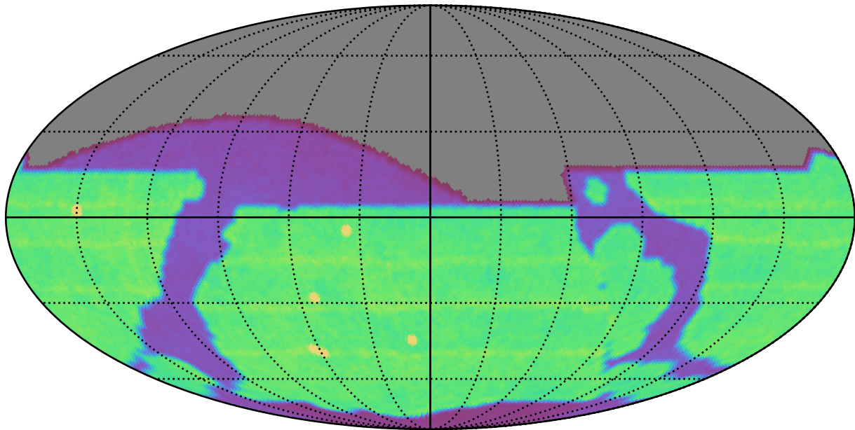
too_elab_r64_d3_gz_v3.4_10yrs All sky all bands: N Unique Nights
