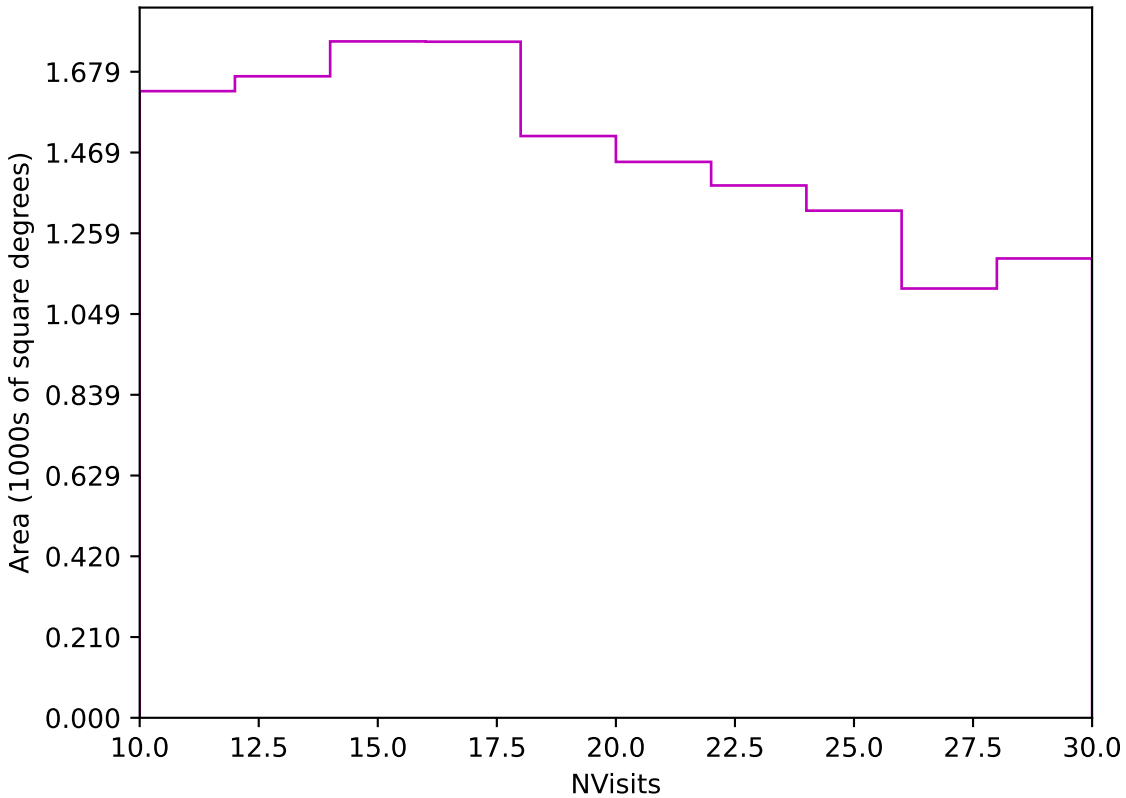
too_elab_r64_d3_gz_v3.4_10yrs Yr 3-4 z band: NVisits
