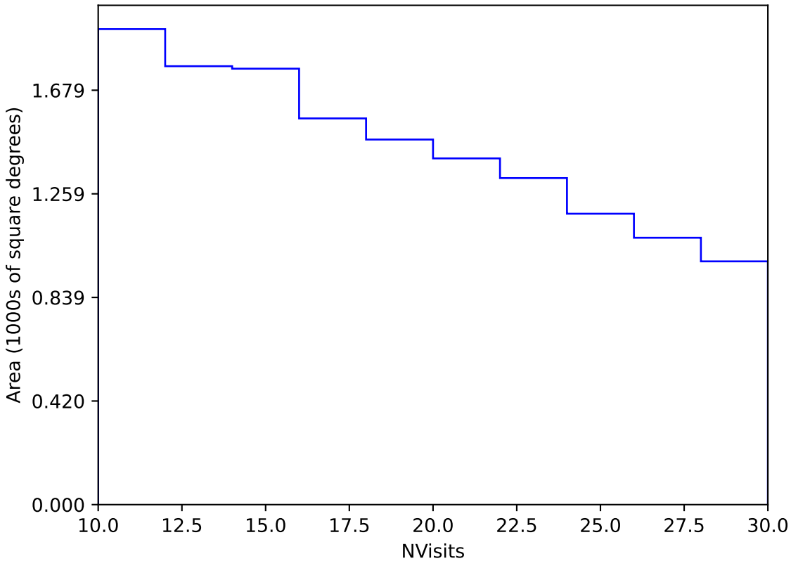
too_elab_r64_d3_gz_v3.4_10yrs Yr 3-4 y band: NVisits
