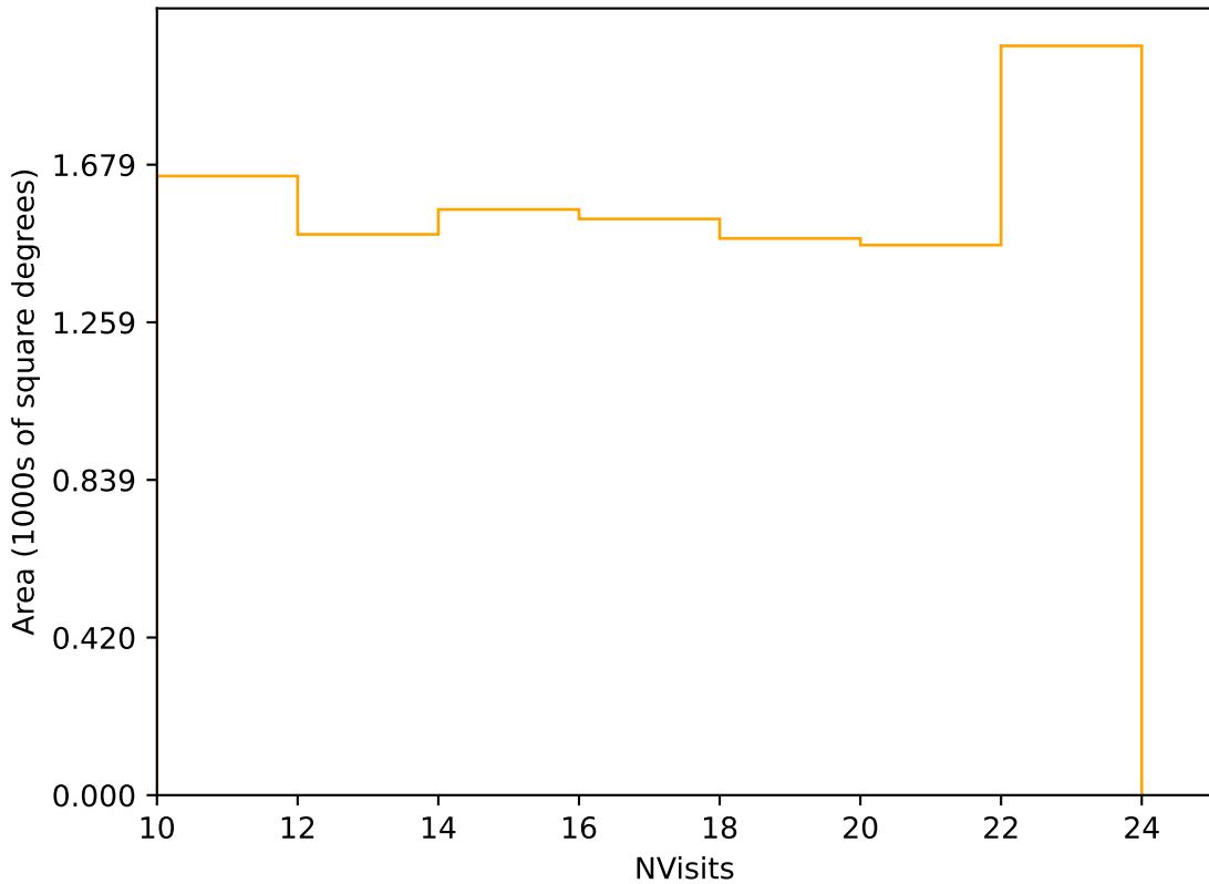
too_elab_r64_d3_gz_v3.4_10yrs Yr 3-4 r band: NVisits
