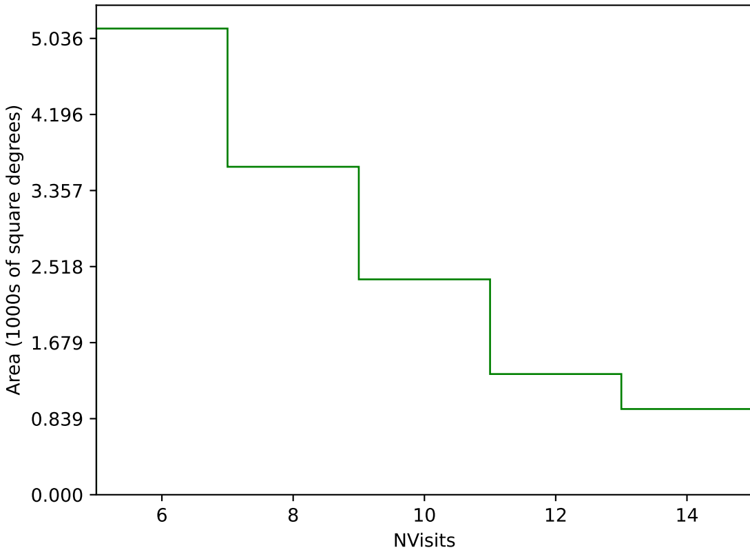
too_elab_r64_d3_gz_v3.4_10yrs Yr 3-4 g band: NVisits
