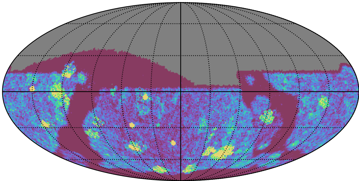
too_elab_r64_d3_gz_v3.4_10yrs Yr 1 z band: NVisits
