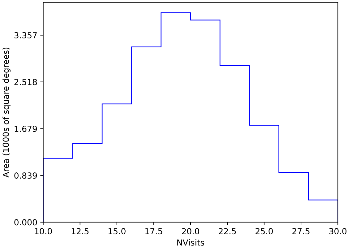
too_elab_r64_d3_gz_v3.4_10yrs Yr 1 y band: NVisits
