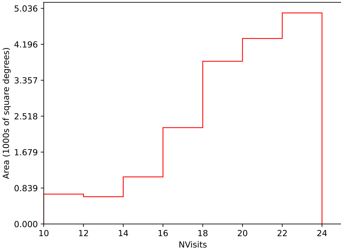
too_elab_r64_d3_gz_v3.4_10yrs Yr 1 i band: NVisits
