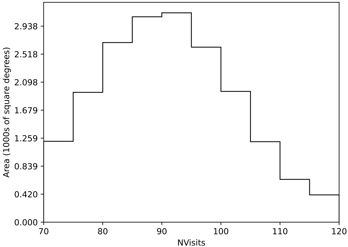
too_elab_r64_d3_gz_v3.4_10yrs Yr 1 all bands: NVisits
