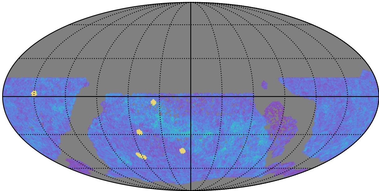
too_elab_r64_d3_gz_v3.4_10yrs WFD z band: NVisits
