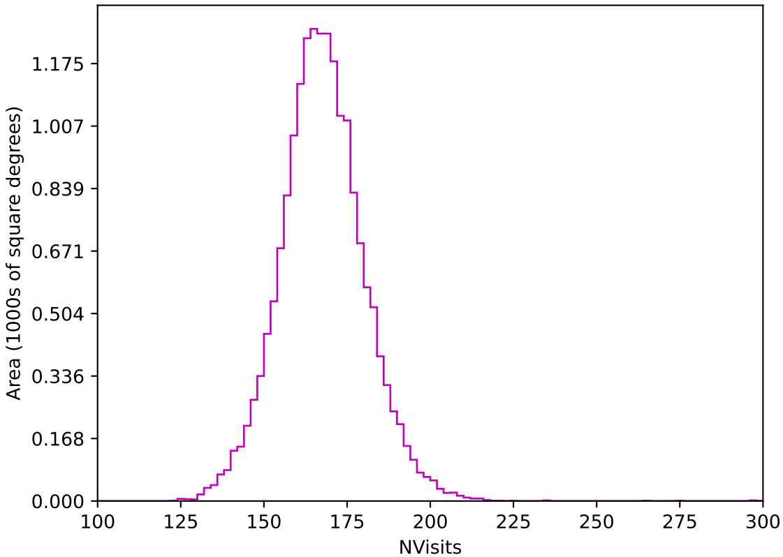
too_elab_r64_d3_gz_v3.4_10yrs WFD z band: NVisits
