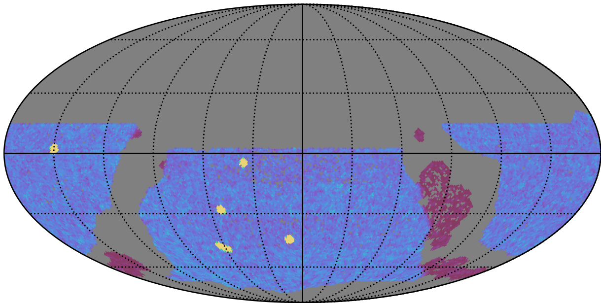
too_elab_r64_d3_gz_v3.4_10yrs WFD y band: NVisits
