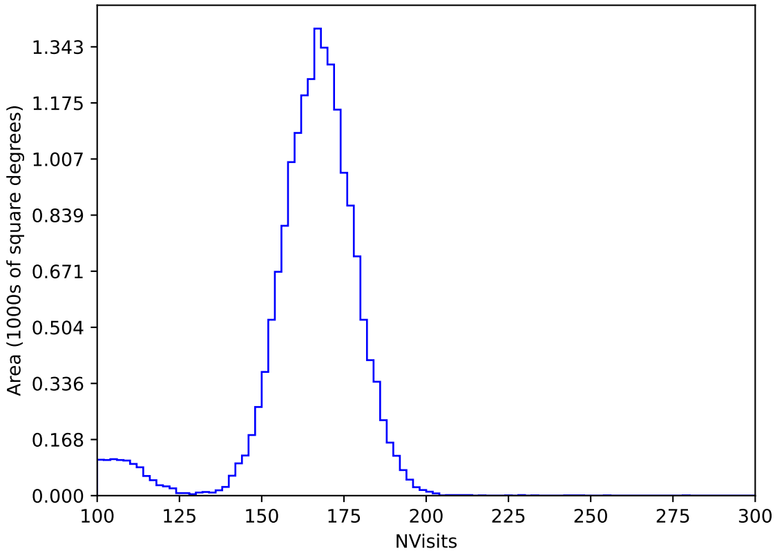
too_elab_r64_d3_gz_v3.4_10yrs WFD y band: NVisits
