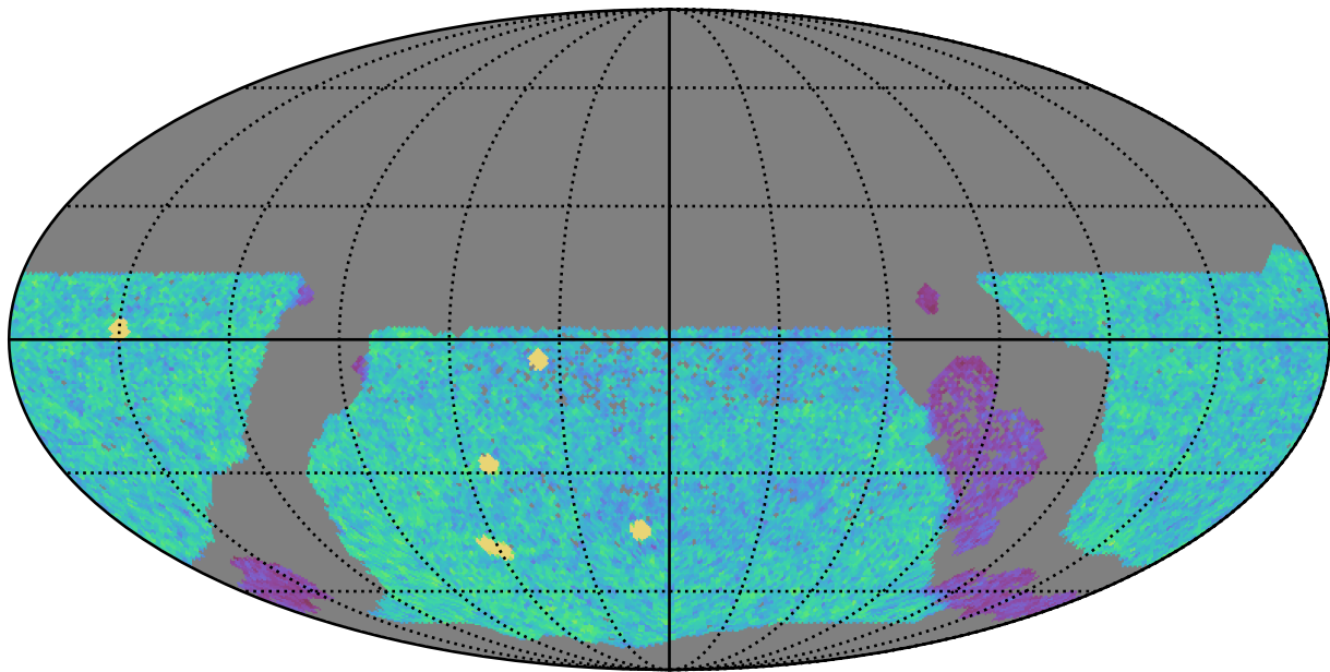
too_elab_r64_d3_gz_v3.4_10yrs WFD u band: NVisits
