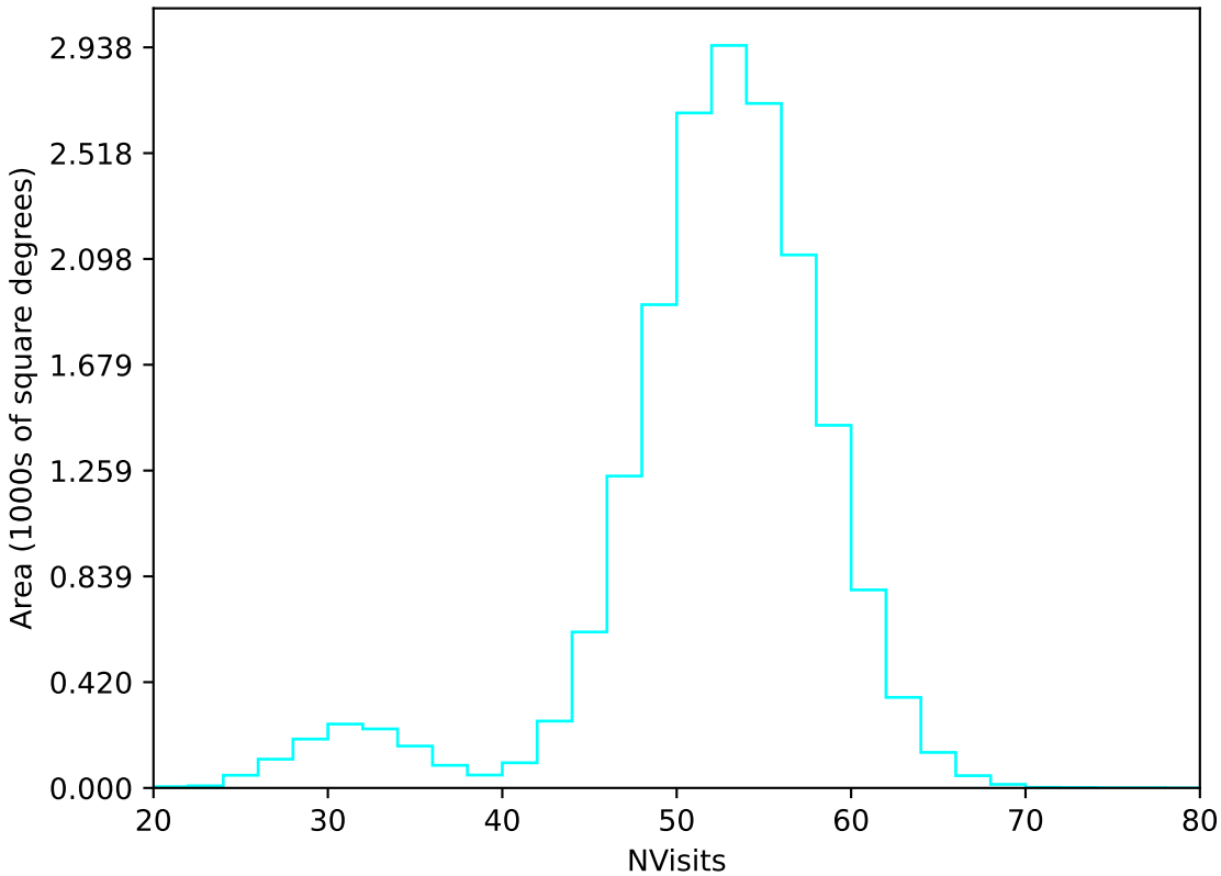
too_elab_r64_d3_gz_v3.4_10yrs WFD u band: NVisits
