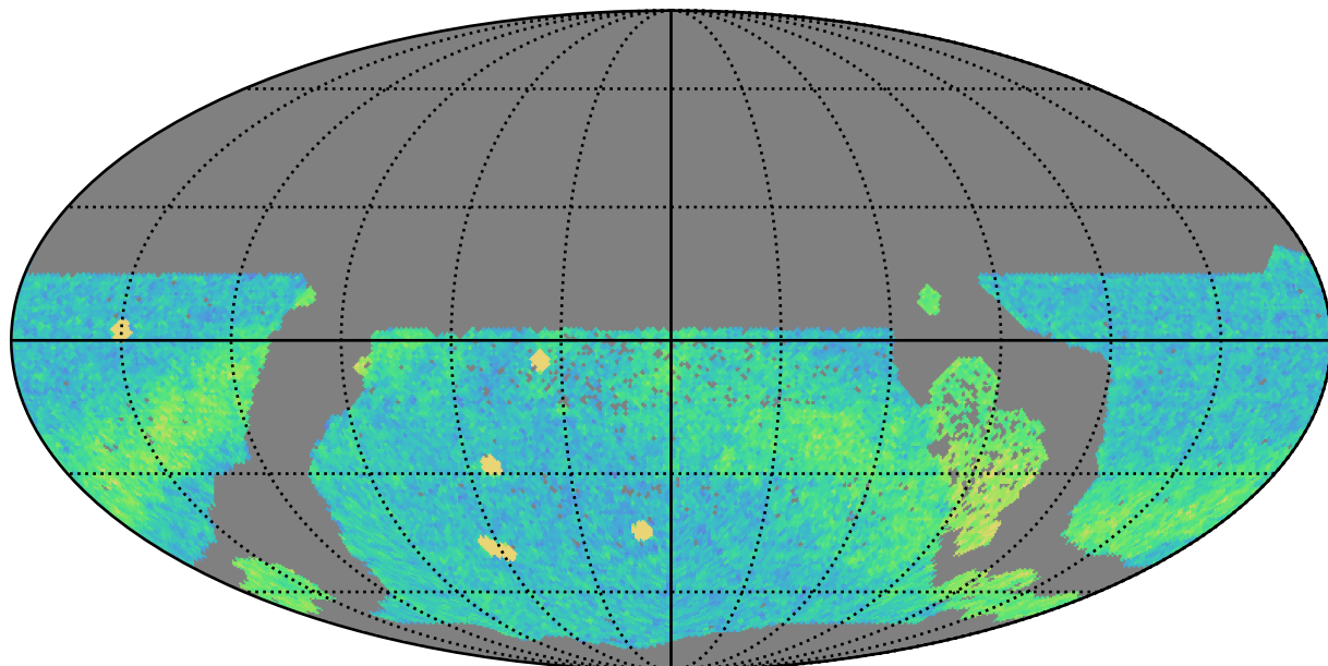
too_elab_r64_d3_gz_v3.4_10yrs WFD r band: NVisits
