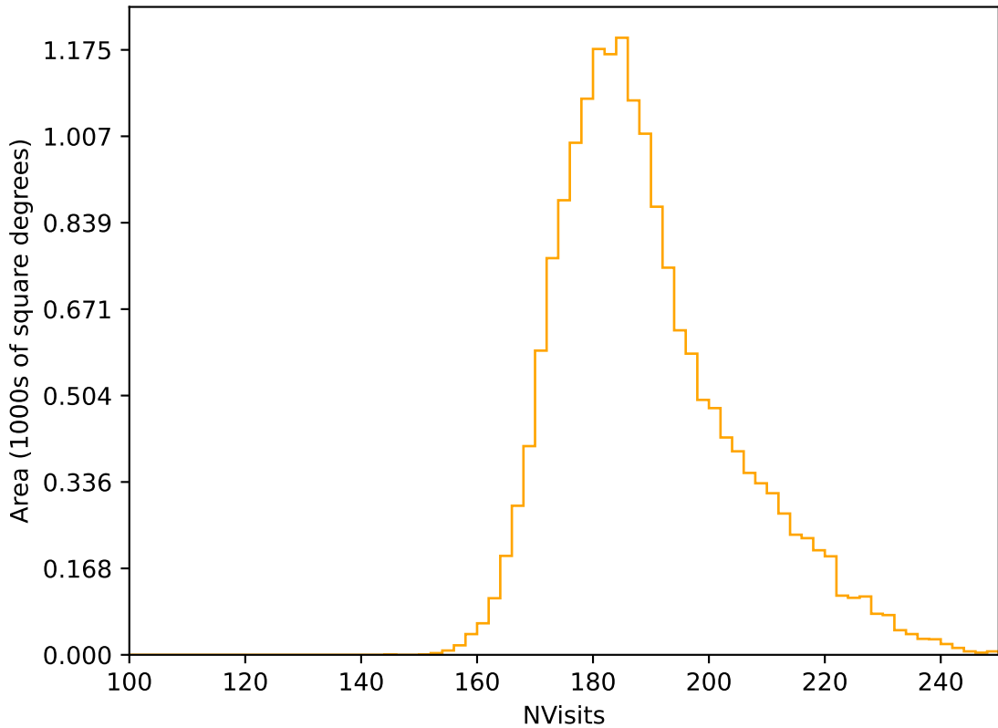
too_elab_r64_d3_gz_v3.4_10yrs WFD r band: NVisits
