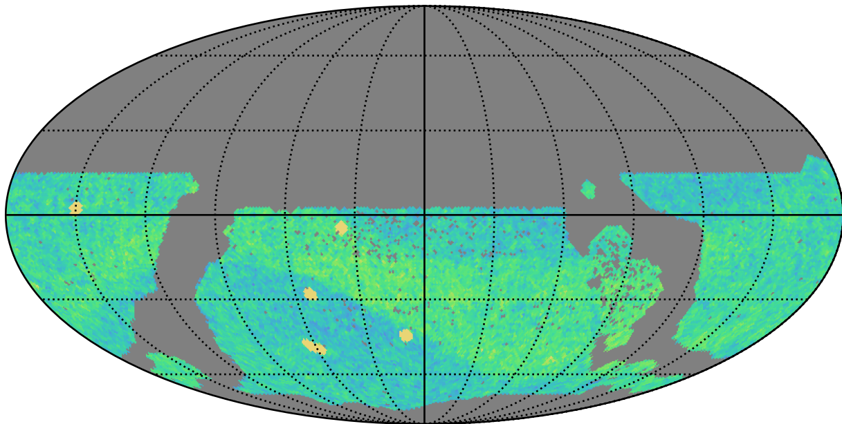
too_elab_r64_d3_gz_v3.4_10yrs WFD i band: NVisits
