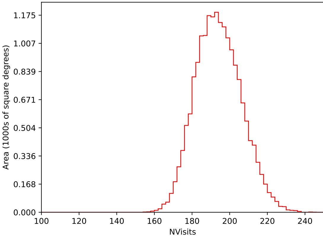
too_elab_r64_d3_gz_v3.4_10yrs WFD i band: NVisits
