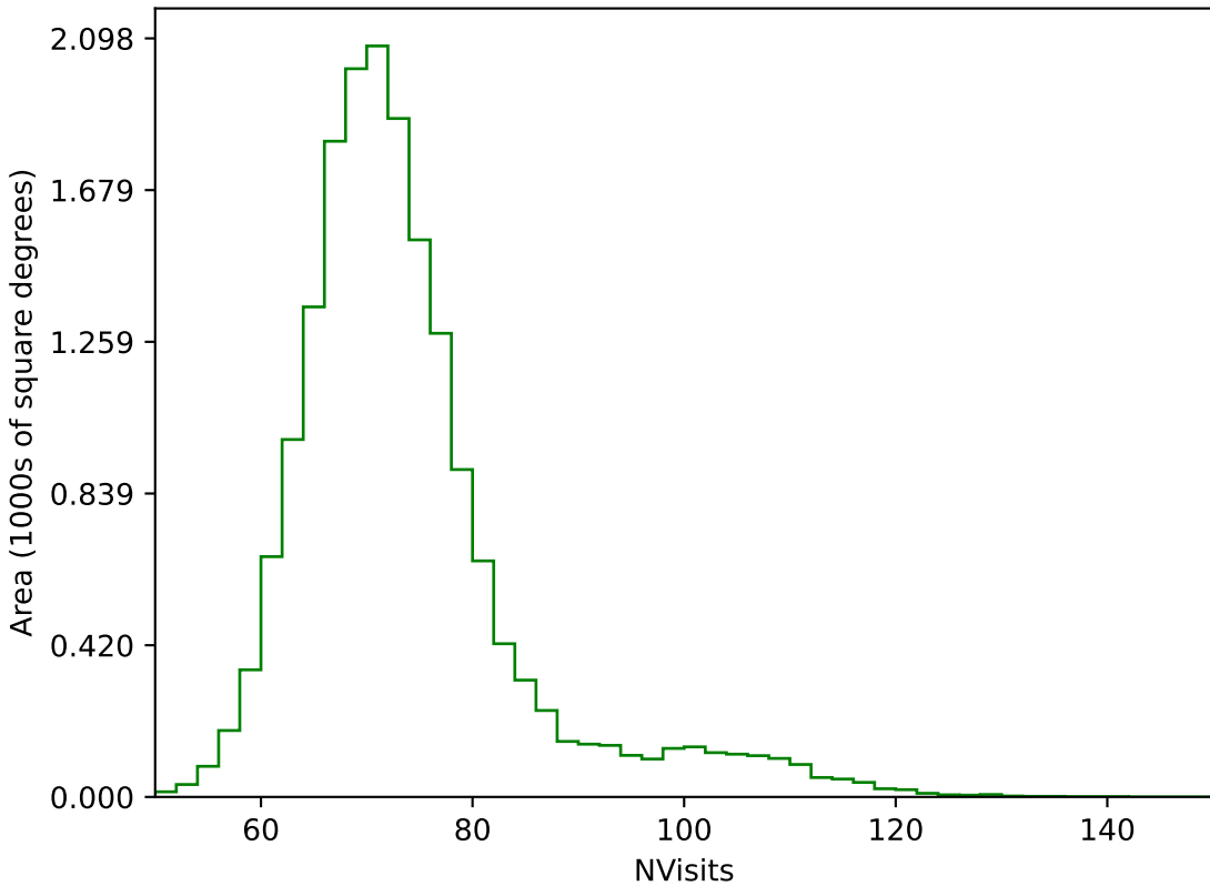
too_elab_r64_d3_gz_v3.4_10yrs WFD g band: NVisits
