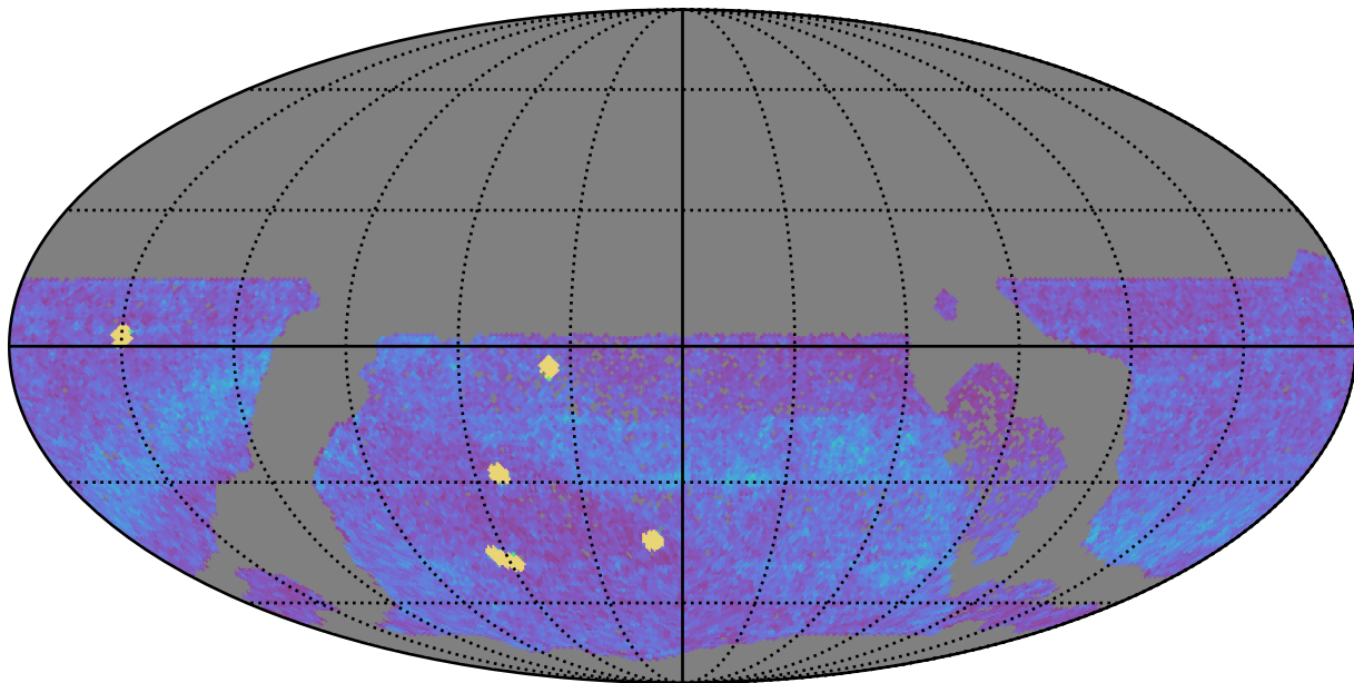
too_elab_r64_d3_gz_v3.4_10yrs WFD all bands: NVisits
