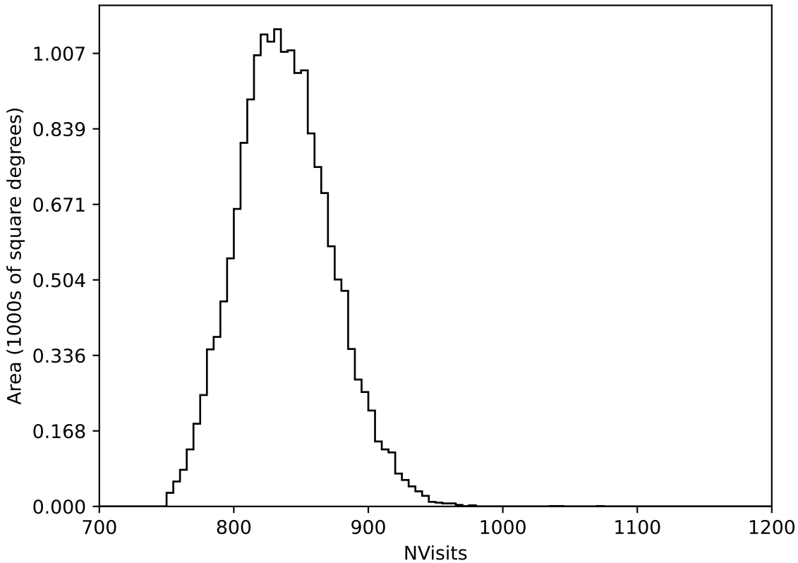
too_elab_r64_d3_gz_v3.4_10yrs WFD all bands: NVisits
