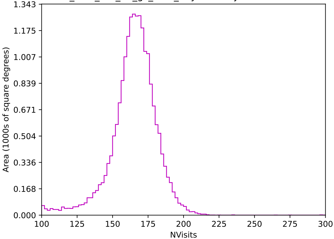
too_elab_r64_d3_gz_v3.4_10yrs All sky z band: NVisits
