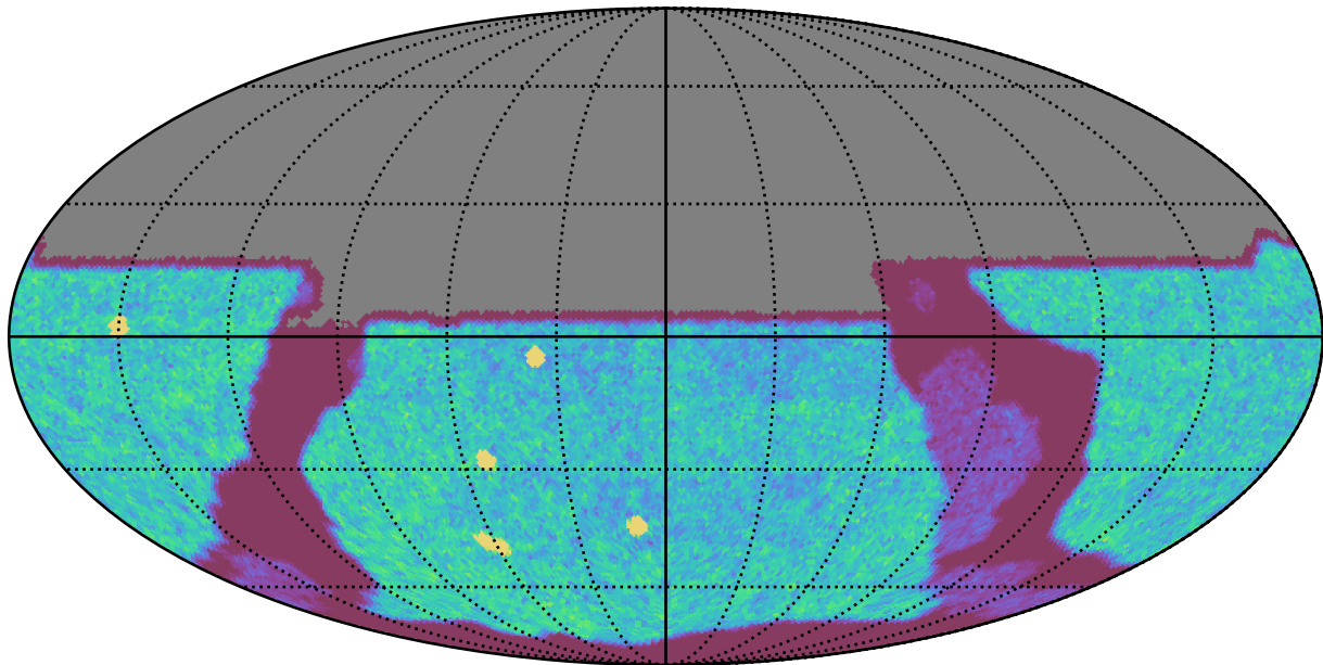
too_elab_r64_d3_gz_v3.4_10yrs All sky u band: NVisits
