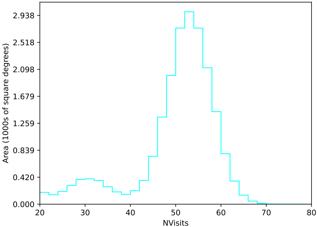
too_elab_r64_d3_gz_v3.4_10yrs All sky u band: NVisits
