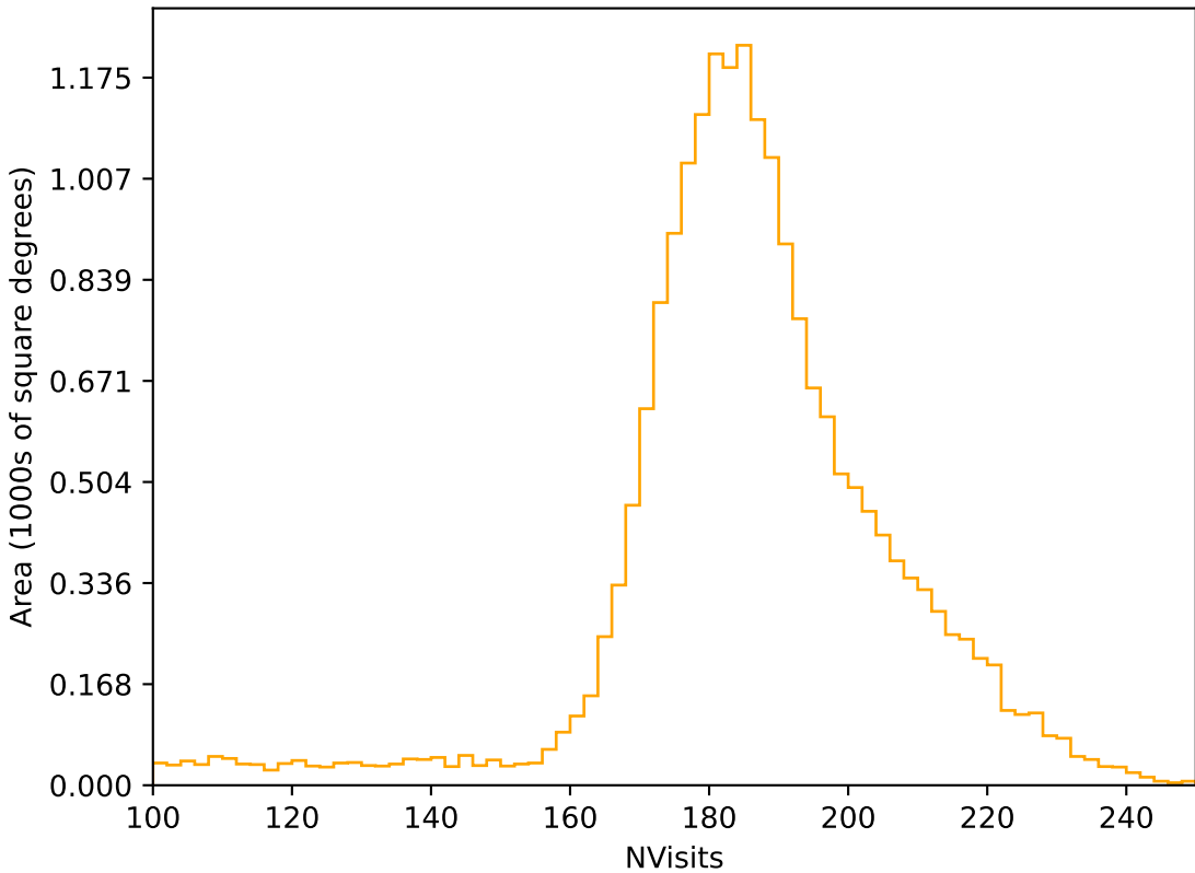
too_elab_r64_d3_gz_v3.4_10yrs All sky r band: NVisits
