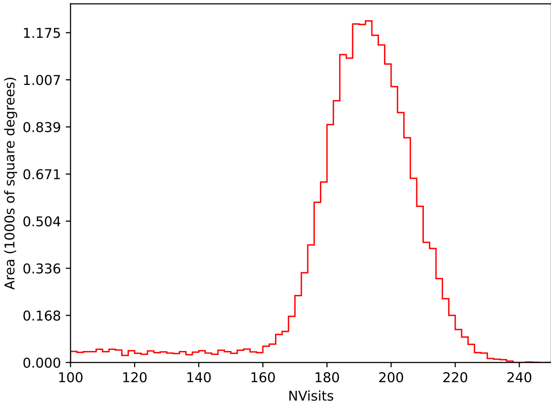
too_elab_r64_d3_gz_v3.4_10yrs All sky i band: NVisits
