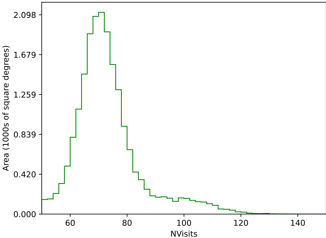
too_elab_r64_d3_gz_v3.4_10yrs All sky g band: NVisits
