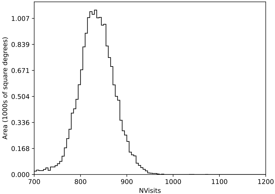
too_elab_r64_d3_gz_v3.4_10yrs All sky all bands: NVisits
