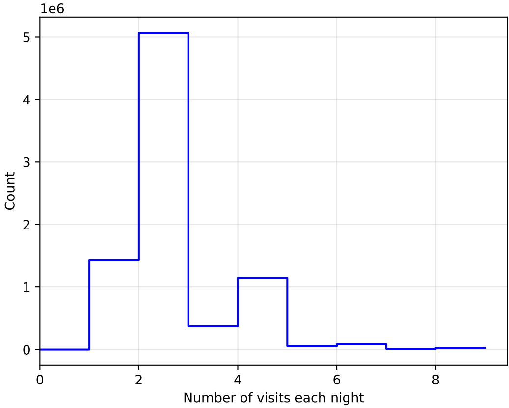
too_elab_r64_d3_gz_v3.4_10yrs WFD: NVisitsPerNight
