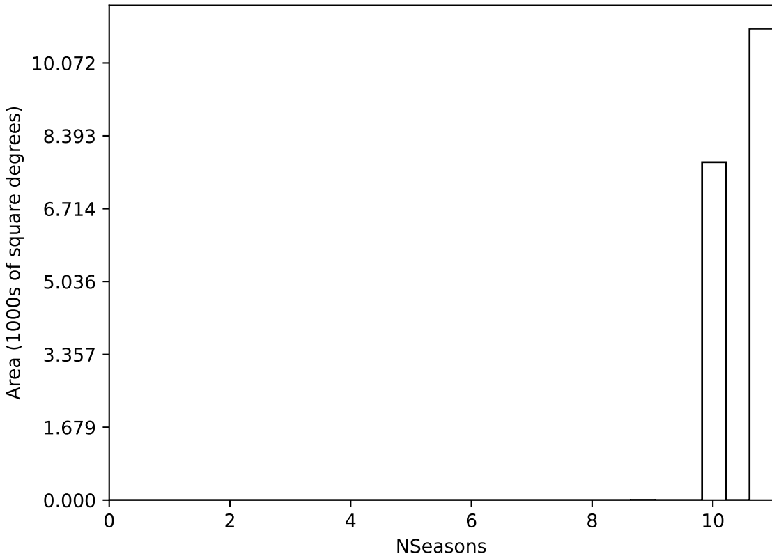
too_elab_r64_d3_gz_v3.4_10yrs WFD all bands: NSeasons
