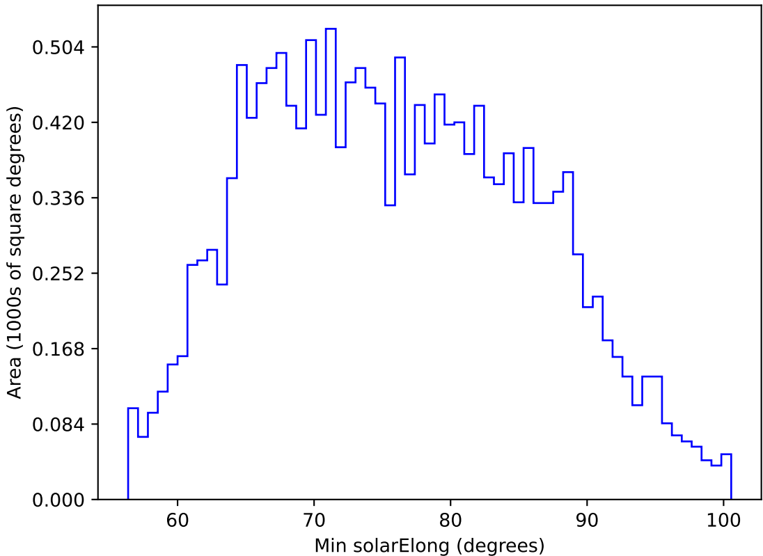
too_elab_r64_d3_gz_v3.4_10yrs WFD u band: Min solarElong
