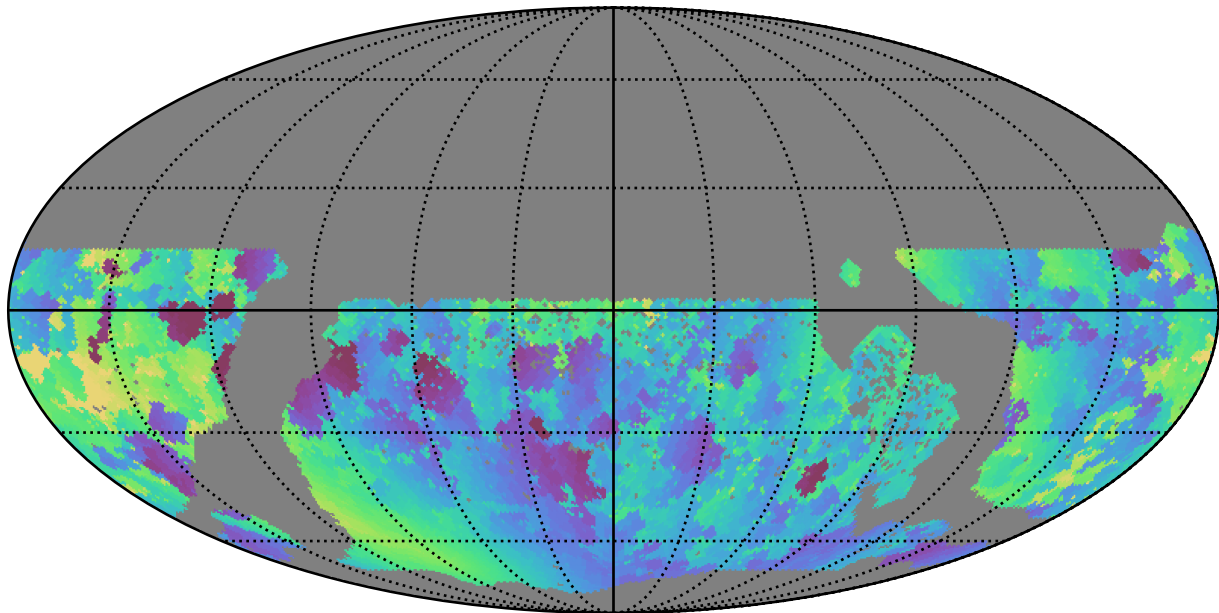
too_elab_r64_d3_gz_v3.4_10yrs WFD g band: Min solarElong
