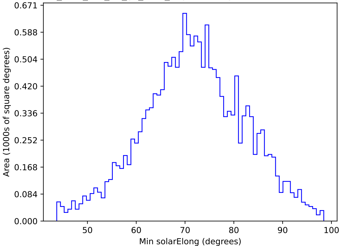
too_elab_r64_d3_gz_v3.4_10yrs WFD g band: Min solarElong
