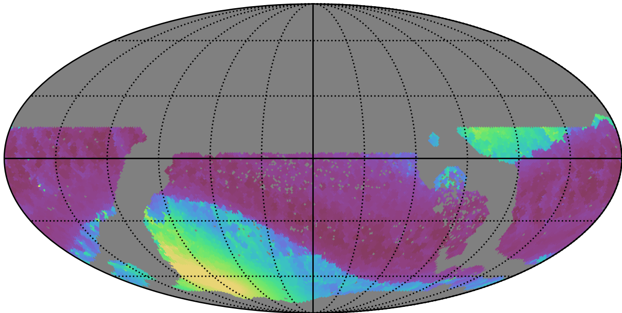
too_elab_r64_d3_gz_v3.4_10yrs WFD all bands: Min solarElong
