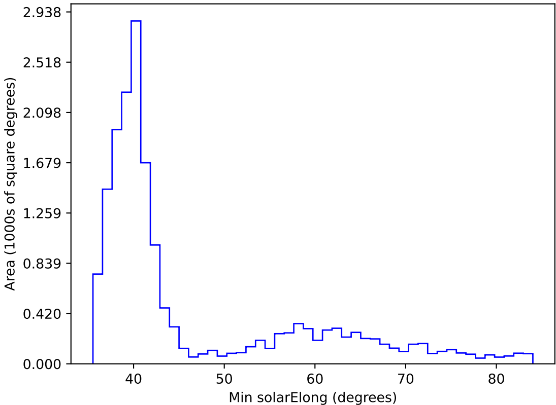
too_elab_r64_d3_gz_v3.4_10yrs WFD all bands: Min solarElong
