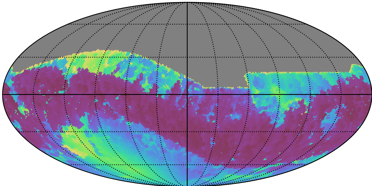
too_elab_r64_d3_gz_v3.4_10yrs All sky z band: Min solarElong
