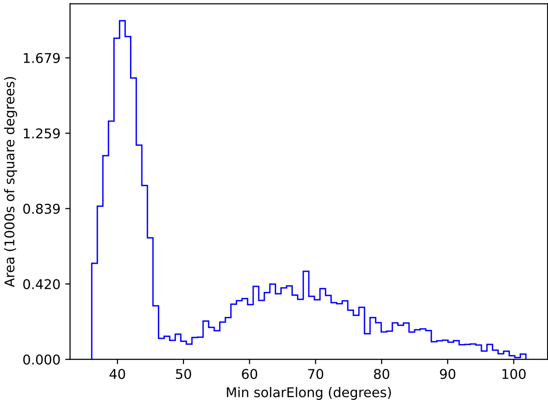
too_elab_r64_d3_gz_v3.4_10yrs All sky z band: Min solarElong
