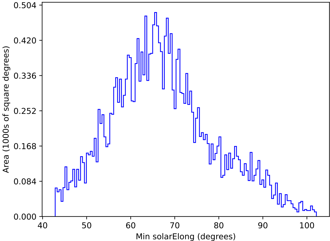
too_elab_r64_d3_gz_v3.4_10yrs All sky y band: Min solarElong
