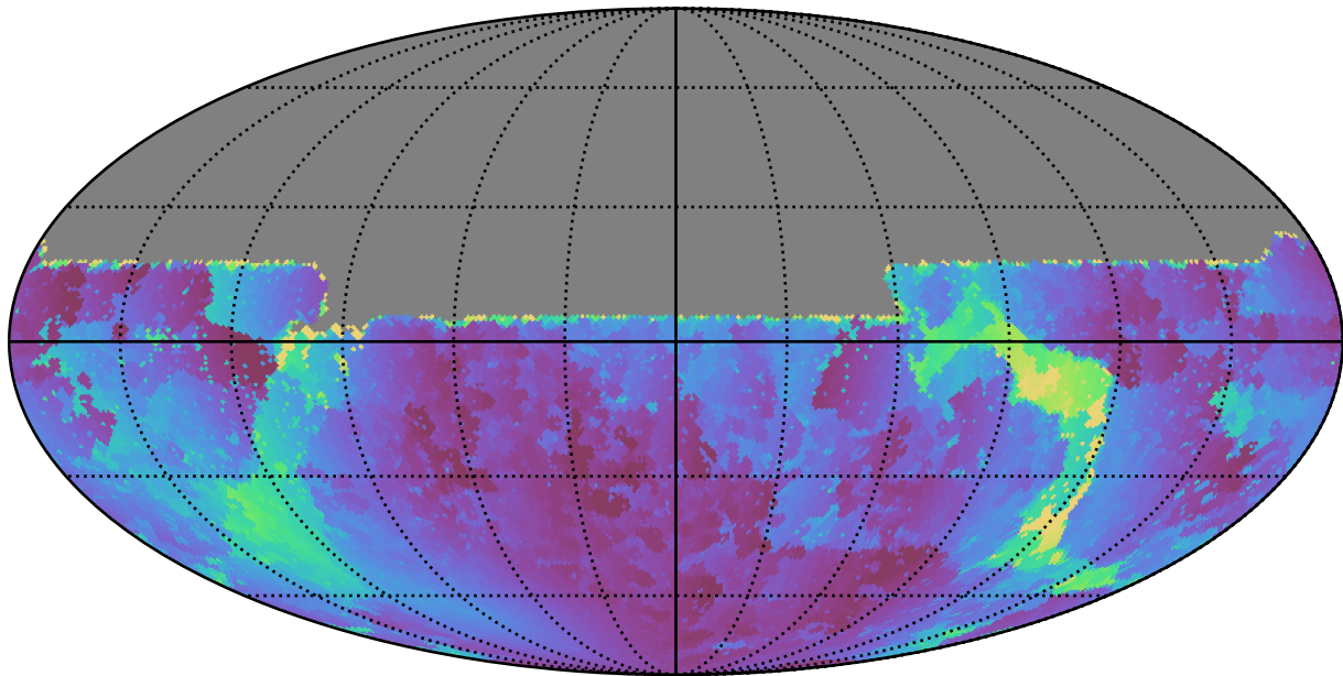
too_elab_r64_d3_gz_v3.4_10yrs All sky u band: Min solarElong
