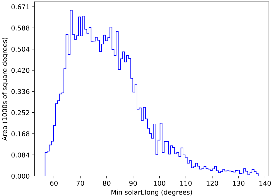
too_elab_r64_d3_gz_v3.4_10yrs All sky u band: Min solarElong
