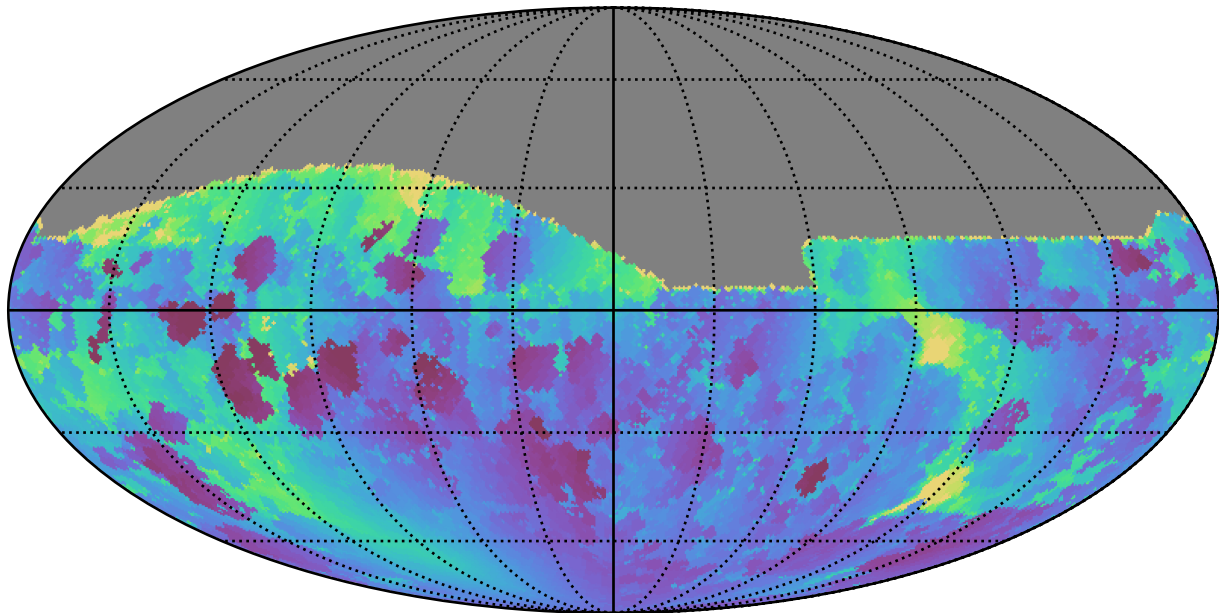
too_elab_r64_d3_gz_v3.4_10yrs All sky g band: Min solarElong
