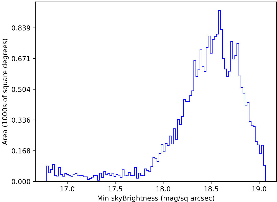
too_elab_r64_d3_gz_v3.4_10yrs Yr 1 z band: Min skyBrightness
