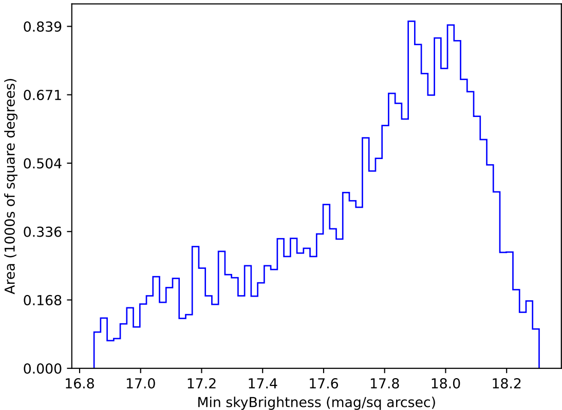
too_elab_r64_d3_gz_v3.4_10yrs Yr 1 y band: Min skyBrightness
