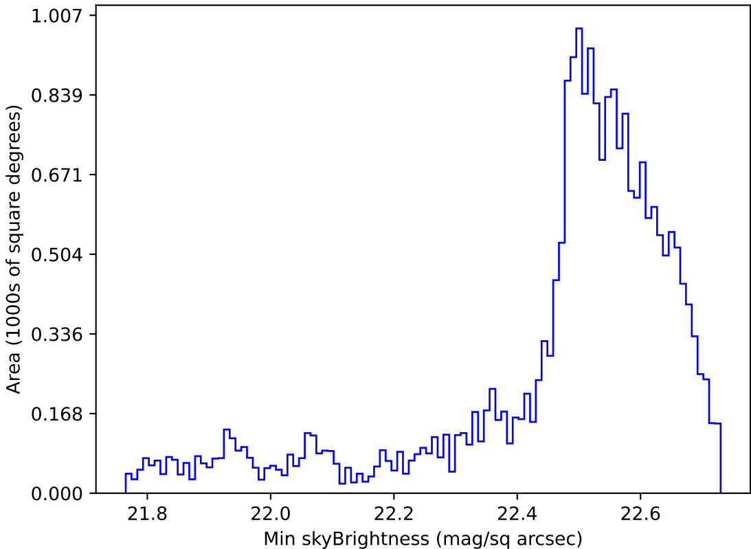
too_elab_r64_d3_gz_v3.4_10yrs Yr 1 u band: Min skyBrightness
