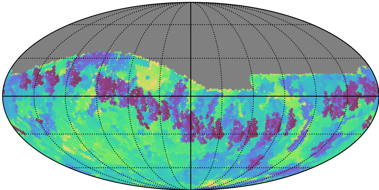
too_elab_r64_d3_gz_v3.4_10yrs Yr 1 i band: Min skyBrightness
